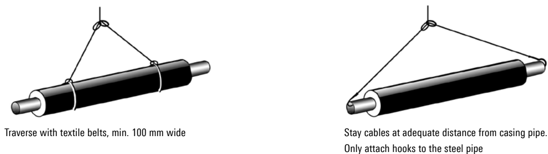
Figure 1: Suspension gear for accident-proof protective handling
