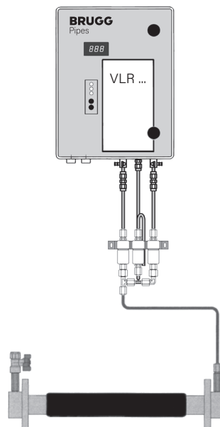
double-walled piping with vacuum leak detector
